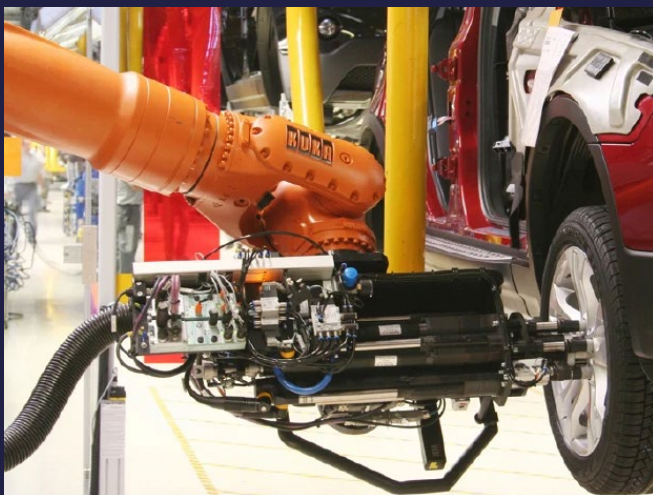
Figure 1: The assembly system mounts wheels onto the continuously moving vehicles
